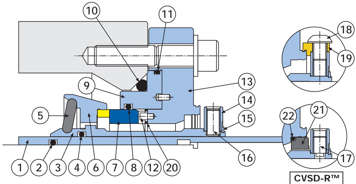
CVSD-R™ Detail showing optional restriction bush.
