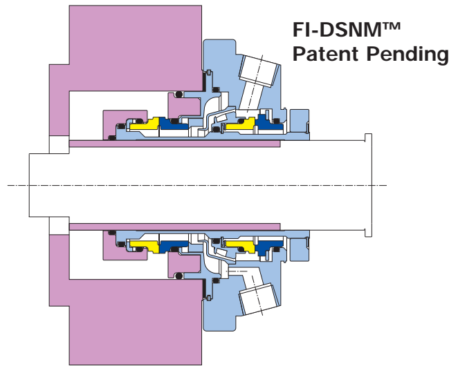
Chemical cartridge double mechanical seal with non-metallic wetted components and optional pumping scroll and wetted elastomers in Kalrez®.
